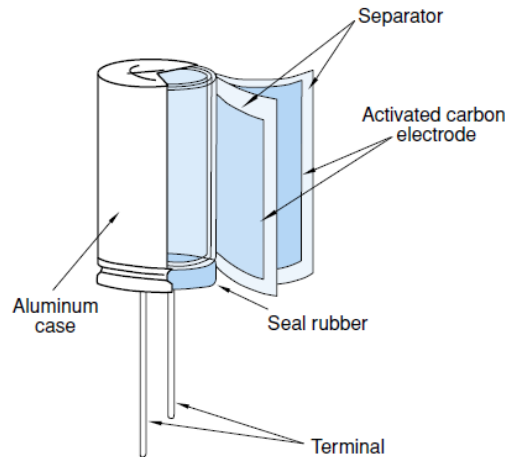
Figure 3: Cell Construction
