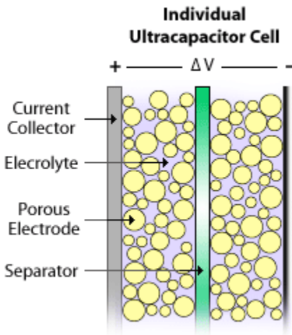
Figure 2: Internal Cell Construction
