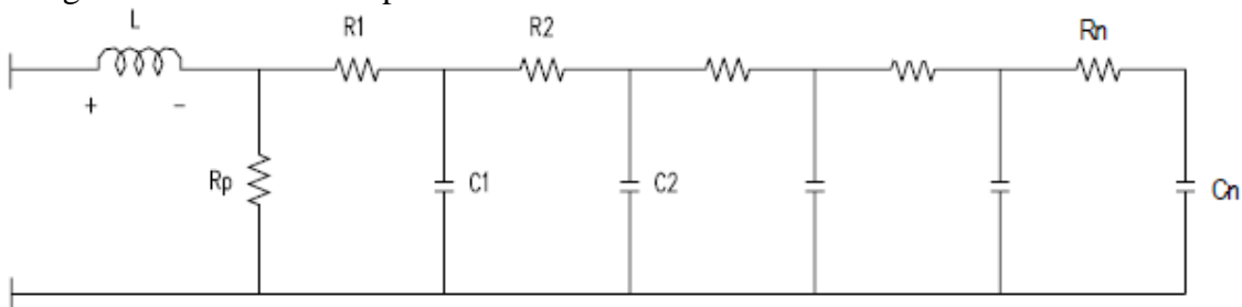
Figure 5: Ladder Network
