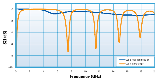
High Q & Broadband MLC Compared Insertion Loss (S21)
