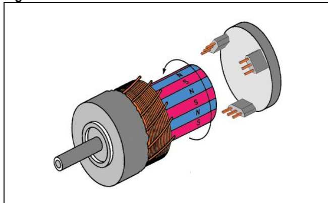
Figure 1. BDCM Sensors
