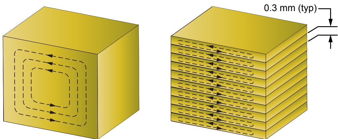
Figure 3. Eddy Currents in Bulk Material (left) and Laminated Material (right). Laminated material has reduced eddy currents.
