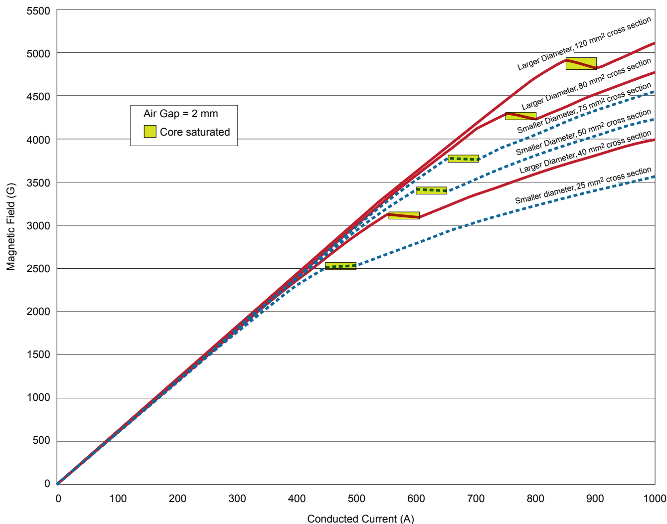
Figure 6. Effects of Core Cross Section and Diameter on the Magnetic Field Flux Density (B). Relative diameter does not significantly affect the magnetic gain, but does affect the magnetic saturation point of the core.
