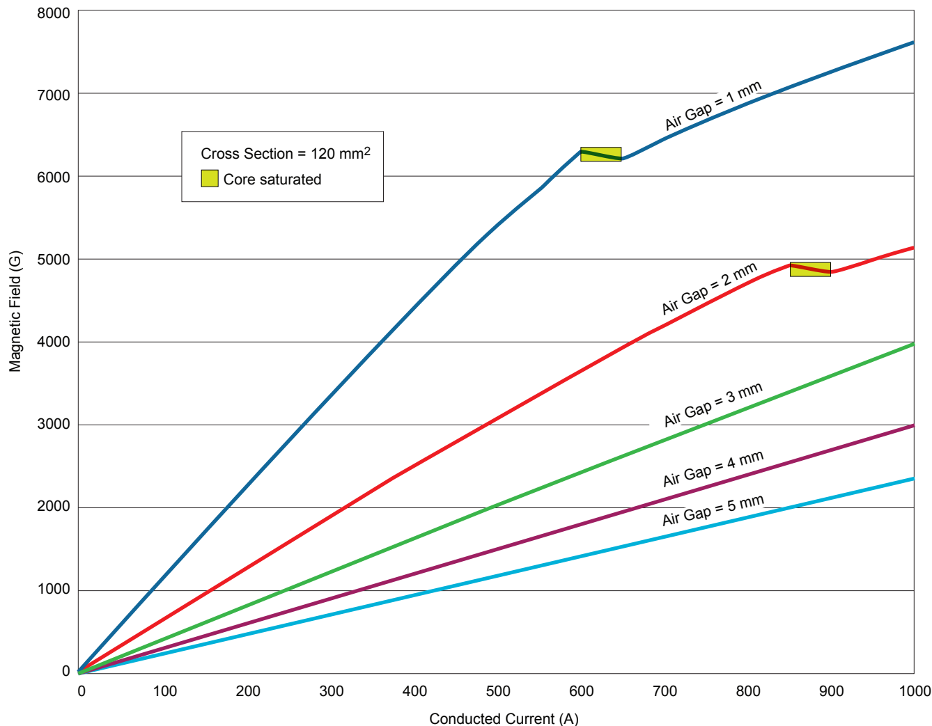
Figure 7. Effects of Air Gap on the Magnetic Field Flux Density (B). Smaller air gaps result in greater magnetic gain, but the saturation points that occur at the smaller air gaps limit current sensing range.
