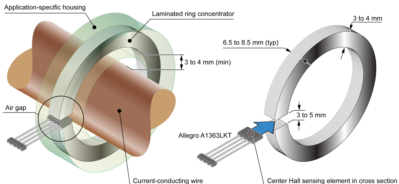
Figure 1. Typical high-current sensing system with concentrator
