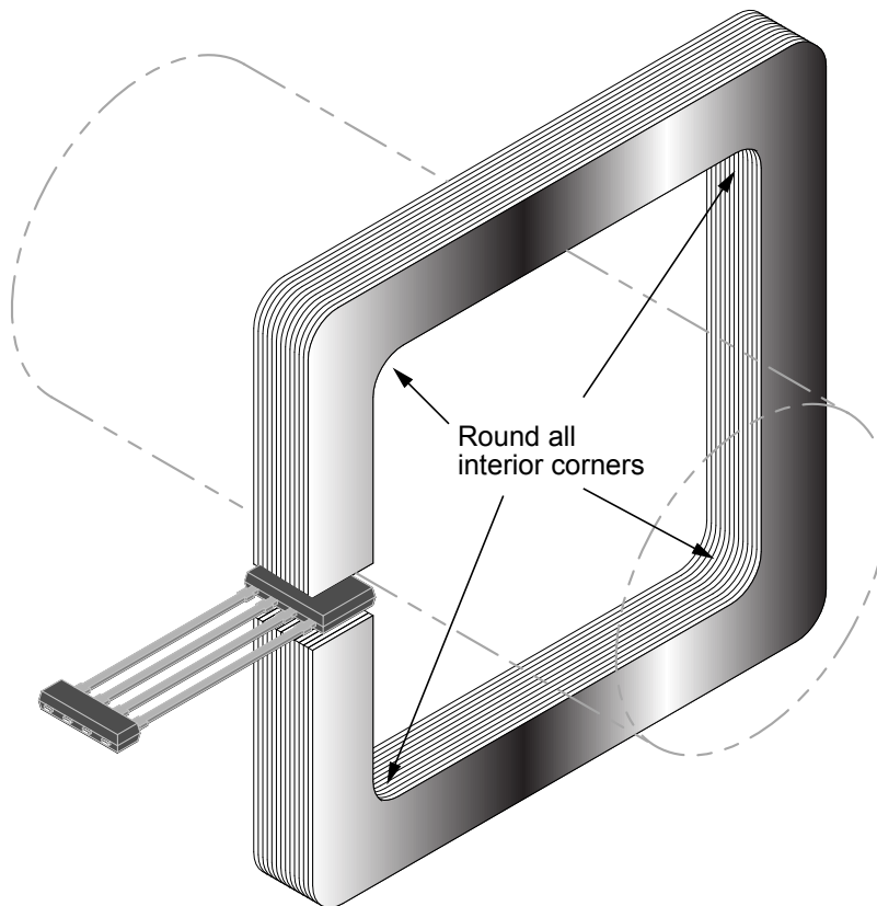
Figure 8. Rectangular Concentrator Configuration. The same design rules apply as with the circular ring concentrators. In addition, the interior corners, and optionally the outer corners, must be rounded to avoid angle effects.
