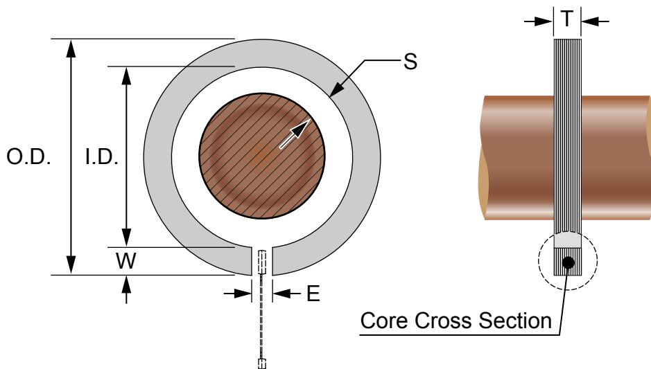
Figure 4. Concentrator Dimensions
