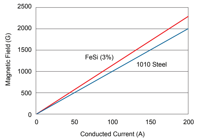
Figure 2. Core Gain for FeSi (3%) and 1010 Steel. For the same core, FeSi generates a higher gain slope (1 G (gauss) = 0.1 mT (millitesla)).
